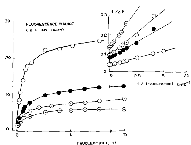
Fig. 3. The dependence of fluorescence change of IAF-enzyme upon the nucleotide concentration (usual plot and double reciprocal plot): (○) AMP; (●) ITP; (◐) GTP; (◑) UTP.
